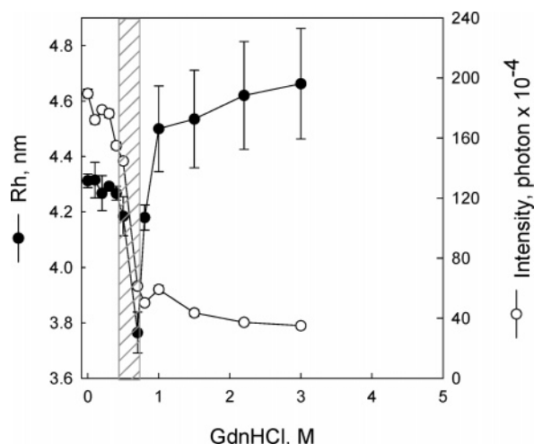
FIGURE 5: Hydrodynamic changes followed by dynamic light scattering. The enzyme was unfolded in the presence of 1 mM MgATP, and the intensity of the dispersed light was recorded (○). The hydrodynamic radius (●) for each sample was calculated from the autocorrelation function obtained from an autocorrelator of 248 channels. The error bars were calculated from 4 measurements. Samples were centrifuged at 13000g before the measurements. Protein concentration was 14 \mu M.
